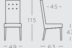
Chair
